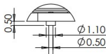
DETAIL A(4:1)
