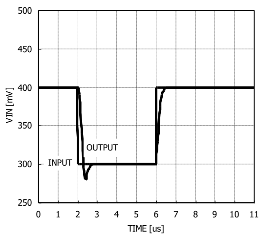
Voltage Follower Pulse Response (Small Signal)
