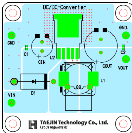
- Top Layout
