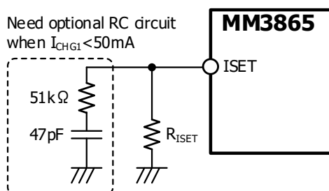
Figure 17. Optional RC circuit at ISET pin
