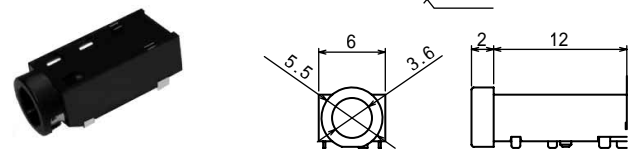
No.MJ-3935-4 (3.5 -4極) SMT 4-CONDUCTOR MINIATURE JACK FOR P.C.B
