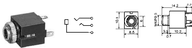
PANEL MOUNT MINIATURE JACK No.MJ-082 (3.5 -3極) No.MJ-083 (3.5 -3極)
