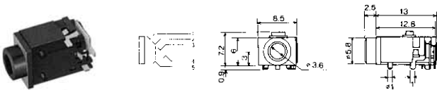
No.MJ-3-249A0 (3.5 -4極) 4-CONDUCTOR MINIATURE JACK FOR P.C.B
