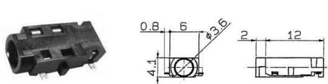
No.M03-992A0 (3.5 -4極) 4-CONDUCTOR MINIATURE JACK FOR P.C.B
