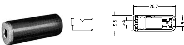
No.MJ-164 (3.5 -2極) MINIATURE INLINE JACK MONO
