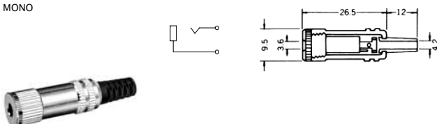
No.MJ-166M (3.5 -2極) MINIATURE INLINE JACK MONO
