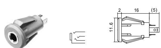
No.MJ-064SP (3.5 -4極) SNAP-IN MOUNT MINIATURE JACK
