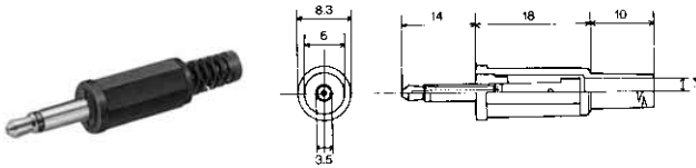
No.MP-106LC (3.5 -2極) 2-CONDUCTOR MINIATURE PLUG w/shielded handle MONO
