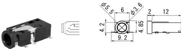
No.MJ-079 (3.5 -4極) 4-CONDUCTOR MINIATURE JACK
