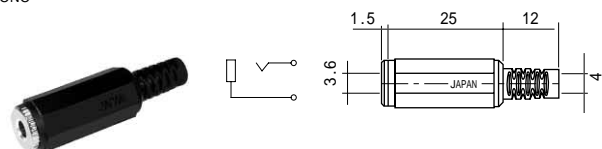
No.MJ-164A (3.5 -2極) MINIATURE INLINE JACK MONO
