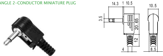
No.MP-105L (3.5 -2極) 2-CONDUCTOR MINIATURE PLUG. MONO
