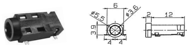
No.M03-992C0 (3.5 -4極) 4-CONDUCTOR MINIATURE JACK FOR P.C.B
