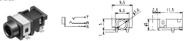
No.M03-772A0 (3.5 -3極) SMT 3-CONDUCTOR MINIATURE JACK FOR P.C.B STEREO
