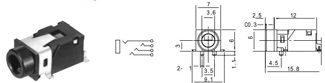
No.MJ-3935-4 (3.5 -4極) SMT 4-CONDUCTOR MINIATURE JACK FOR P.C.B
