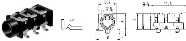
No.MJ-4435 (3.5 -3極) SMT 3-CONDUCTOR MINIATURE JACK FOR P.C.B STEREO
