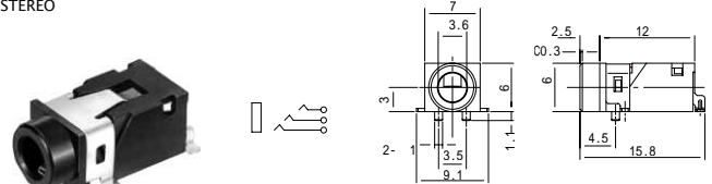
No.MJ-3935-3 (3.5 -3極) SMT 3-CONDUCTOR MINIATURE JACK FOR P.C.B STEREO
