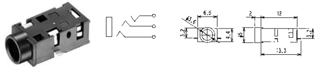
No.M03-836F0 (3.5 -3極) SMT 3-CONDUCTOR MINIATURE JACK FOR P.C.B STEREO
