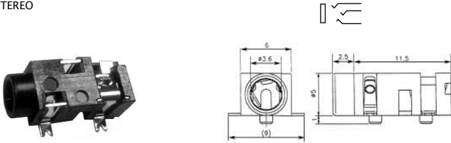
No.MJ-073SP (3.5 -3極) SNAP-IN MOUNT MINIATURE JACK STEREO
