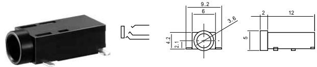
No.MJ-3935-3 (3.5 -3極) SMT 3-CONDUCTOR MINIATURE JACK FOR P.C.B STEREO
