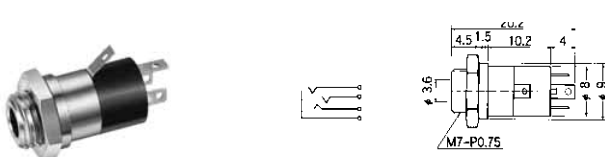
No.MJ-079 (3.5 -4極) 4-CONDUCTOR MINIATURE JACK
