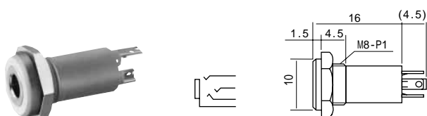
No.MJ-064H (3.5 -4極) PANEL MOUNT MINIATURE JACK
