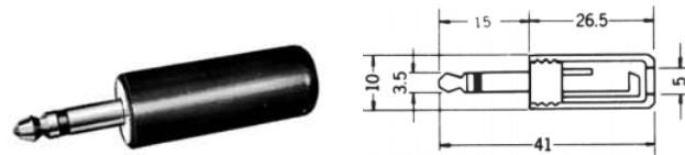
No.MP-105L (3.5 -2極) 2-CONDUCTOR MINIATURE PLUG. MONO
