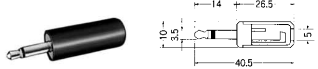
No.MP-105LC (3.5 -2極) 2-CONDUCTOR MINIATURE PLUG MONO
