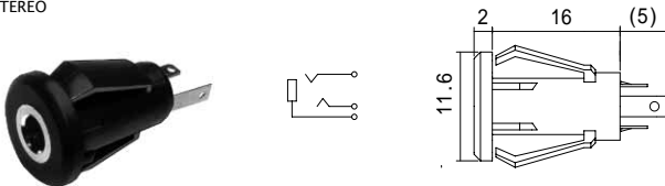
No.MJ-073SP (3.5 -3極) SNAP-IN MOUNT MINIATURE JACK STEREO
