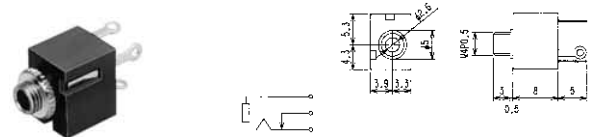
No.MJ-255 (2.5 -2極) PANEL MOUNT SUB-MINIATURE JACK MONO
