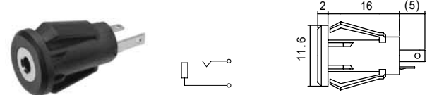
No.MJ-165SP (2.5 -2極) SNAP-IN MOUNT SUB-MINIATURE JACK MONO
