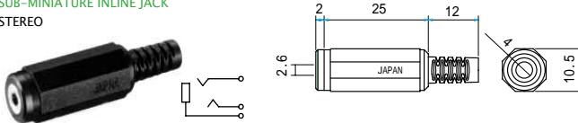
No.MJ-0253S (2.5 -3極) 3-CONDUCTOR SUB-MINIATURE INLINE JACK STEREO
