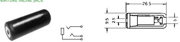
No.MJ-071 (2.5 -3極) SUB-MINIATURE INLINE JACK STEREO
