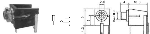
No.MJ-147D (2.5 -2極) 2-CONDUCTOR SUB-MINIATURE JACK FOR P.C.B MONO
