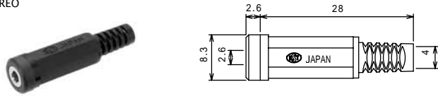
No.MJ-0253S (2.5 -3極) 3-CONDUCTOR SUB-MINIATURE INLINE JACK STEREO
