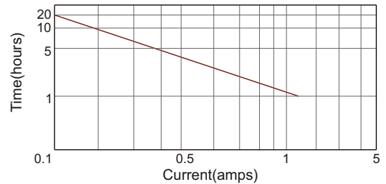
Discharge current v's time 77°F(25°C)
