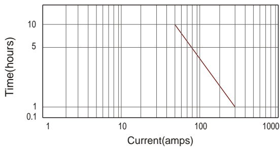
Discharge current v's time 77°F(25°C)
